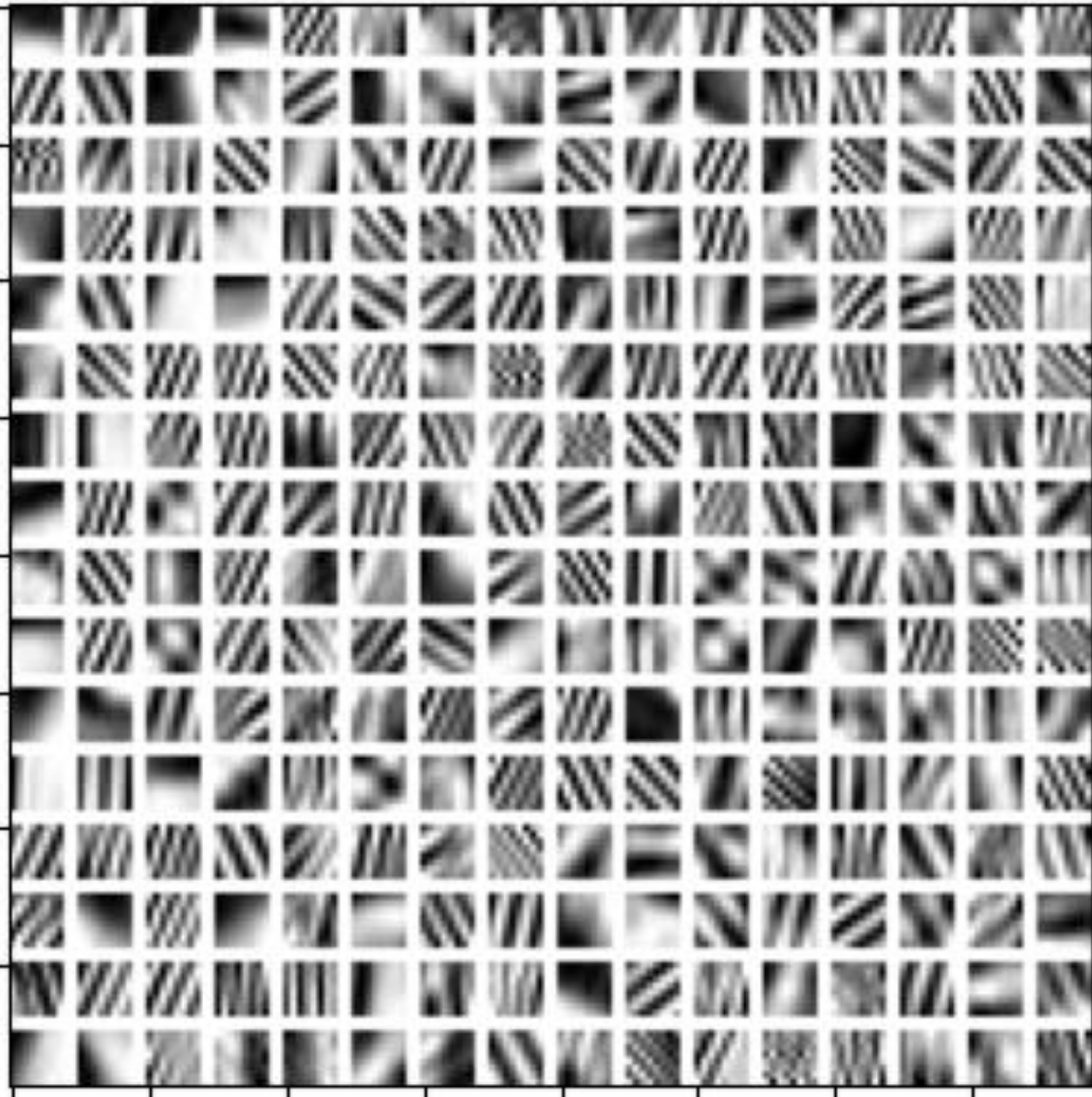
Learned Dictionary
