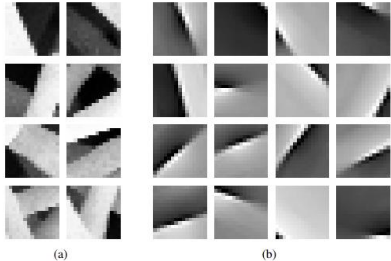
Learned Dictionary
