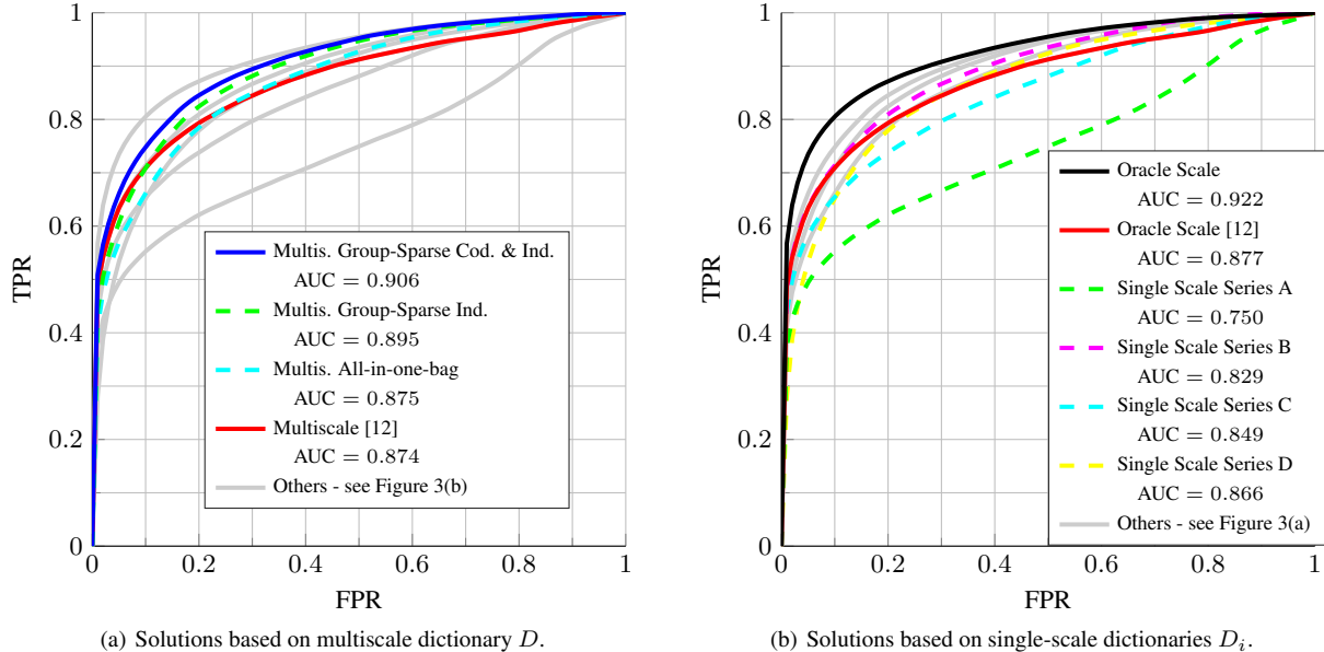
Fig. 3. ROC curves for all methods presented in Section 4. (a) the ROC curves of solutions based on the multiscale dictionary D (3); (b) the ROC curves of solutions based on single scale dictionary D_i . There are 4 ROC curves for single scale dictionaries: one for each series of images used in the training phase. The area under the curve (AUC) of each ROC curve is reported in the legend.
